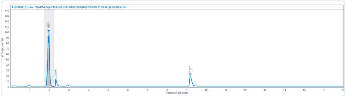
HPLC Chromatogram · Retention Time 1.965, 2.316, 9.182 min
