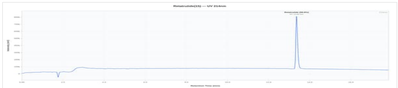
Retatrutide 15 - 3-26-002: UV Chromatogram
