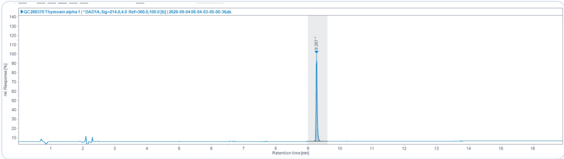
HPLC Chromatogram · Retention Time 9.267 min
